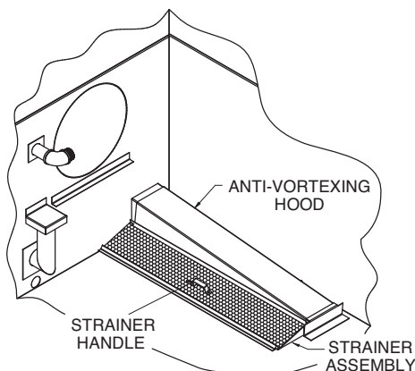
Figure 14 – LSTE/PMTQ Strainer Assembly
