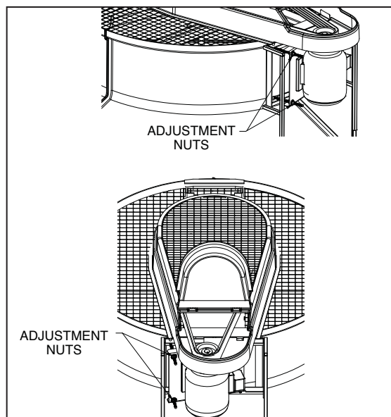
Figure 6 – MTT Shaft-Up Mounted Motors
