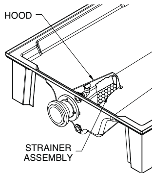
Figure 14 – MTT V-Sump Strainer Assembly
