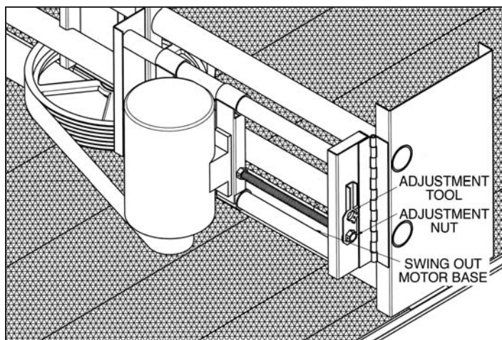
Figure 7 – AT, UT, USS, UAT, cAT Internally Mounted Motors
