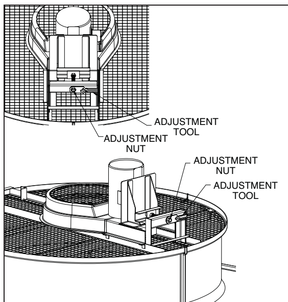
Figure 5 – MTT Top Mounted Motors
