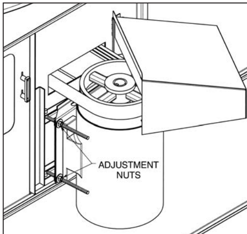
Figure 3 – AT, UT, USS, UAT, cAT Externally Mounted Motors
