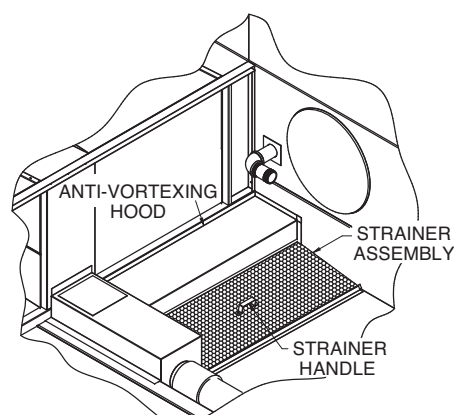
Figure 15 – LPT Strainer Assembly
