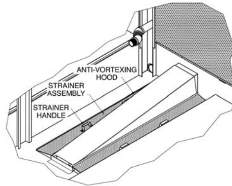
Figure 11 – AT, UT, USS, UAT, cAT Dual Strainer Assembly
