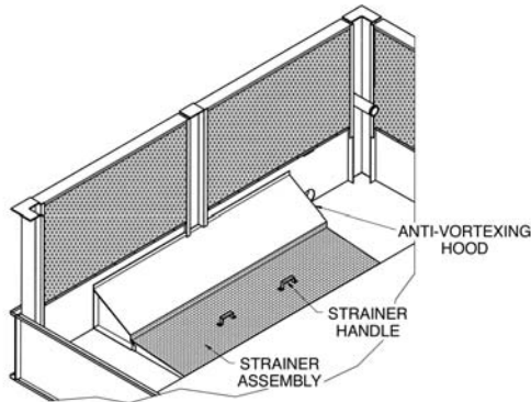
Figure 10 – AT, UT, USS, UAT, cAT Single Strainer Assembly
