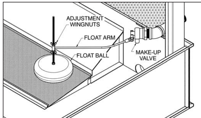
Figure 16 – Mechanical Water Make Up Valve
