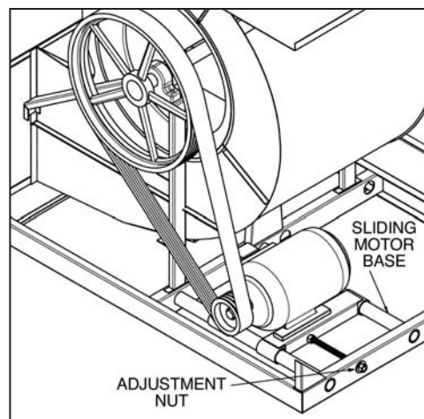
Figure 8 – LPT Motor Adjustment
