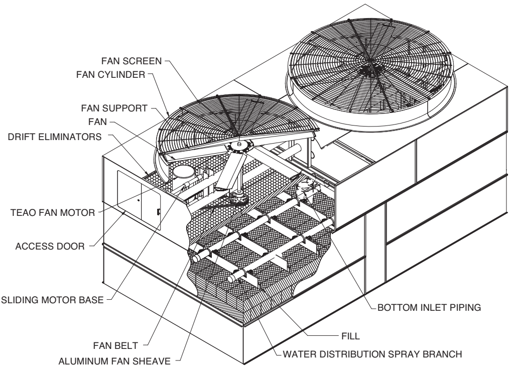
FAN & FILL CASING SECTION (ONE CELL SHOWN)
