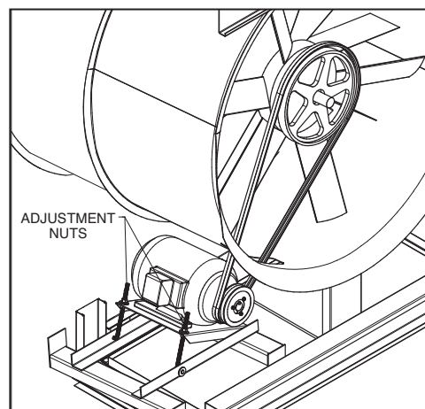
Figure 9 – PM Style Motor Adjustment
